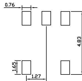
Recommended PAD Layout Top View
