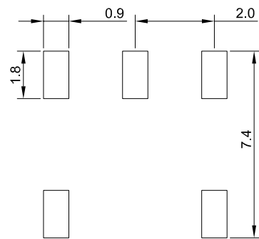
Recommend Pad layout
